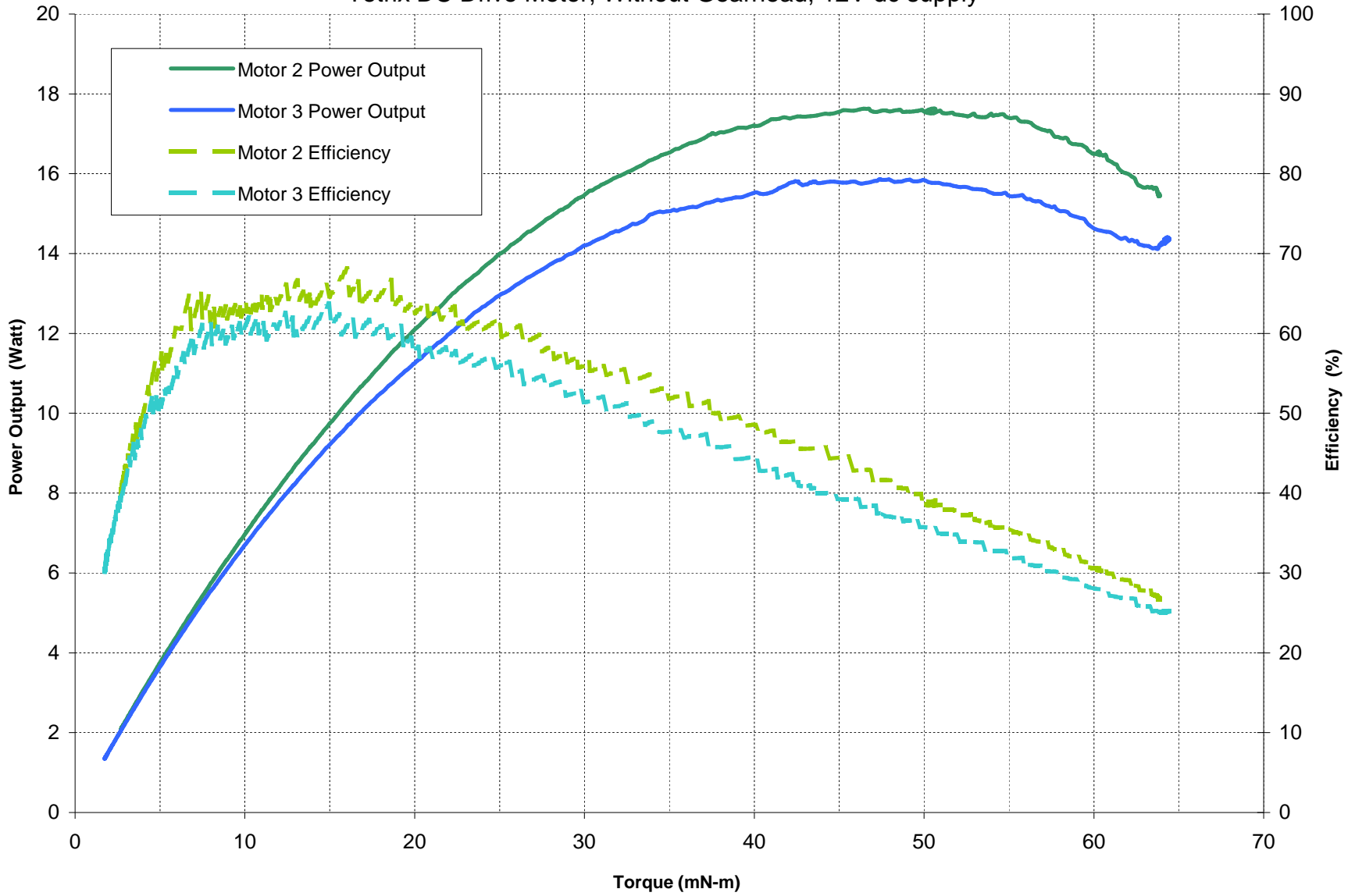
Tetrix DC Drive Motor, Without Gearhead, 12V dc supply
